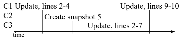
FIGURE 2—Execution trace exposing a bug in the Figure 1 code. Client C1, a slow updater, performs update lines 2–4, looking up a certain key and finding version #5. Since the last snapshot epoch is #4, the object is up to date and no copy-on-write is needed so it skips to line 9. Update lines 9–10, which happen later, update the current table with new contents but still version #5. Meanwhile, client C2 creates a new snapshot, and client C3 does an update involving a copy-on-write to snapshot table #5. At the end of this trace, the snapshot invariant is violated: snapshot table #5 contains contents that do not reflect the latest update, just performed by C1.
